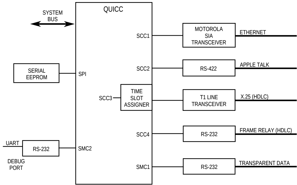
Figure 1-20. General-Purpose Application
