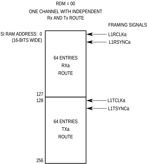
Figure 7-23. SI RAM: One TDM with Static Frames
