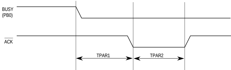
Figure 7-89. Centronics Receiver Timing Mode 0
