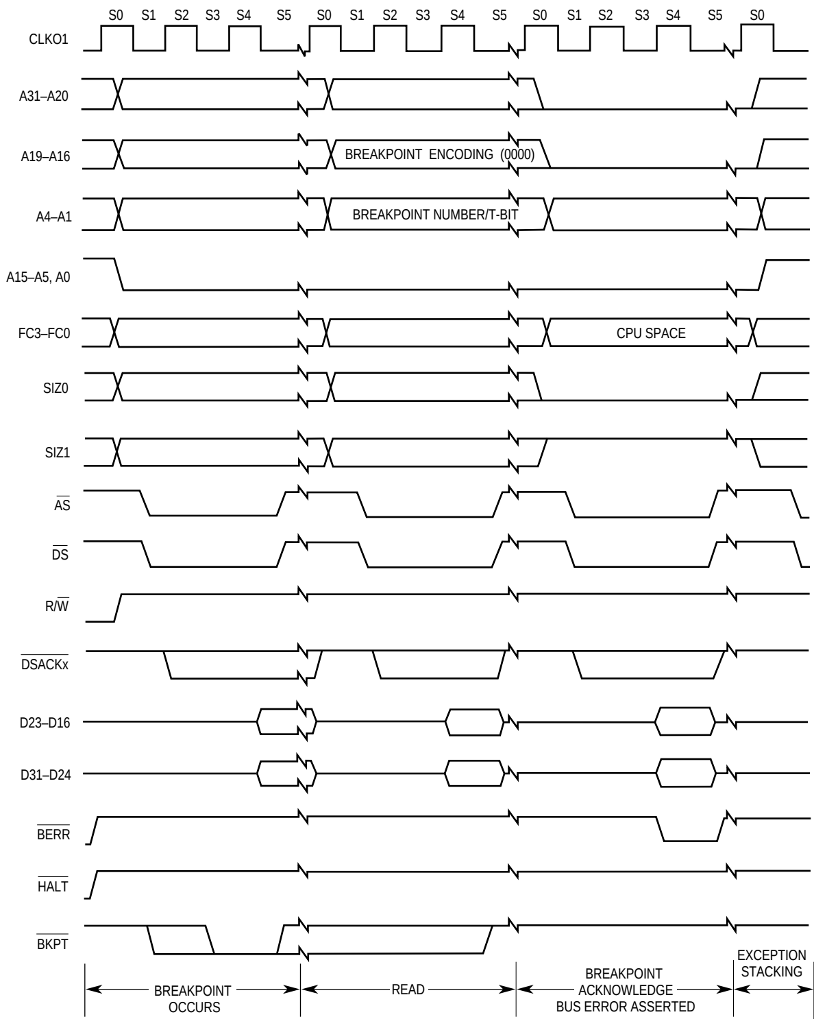
Figure 4-25. Breakpoint Acknowledge Cycle Timing (Exception Signaled)
