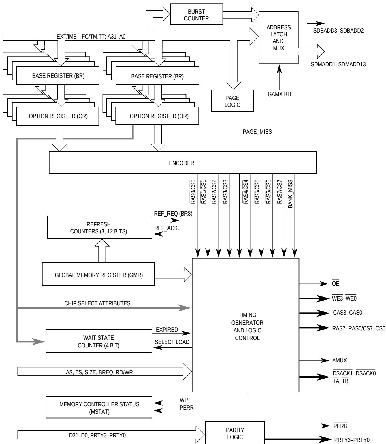
Figure 6-10. Memory Controller Block Diagram
