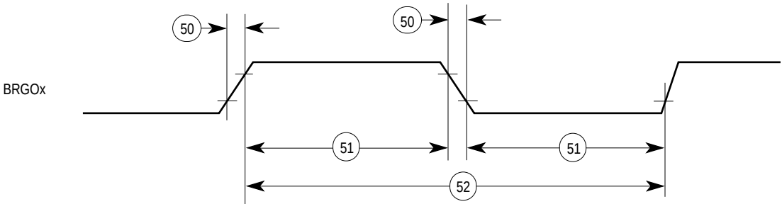
Figure 10-58. Baud Rate Generator Output Signals
